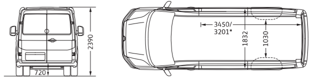
Crafter 50/55 Van LWB High Roof
