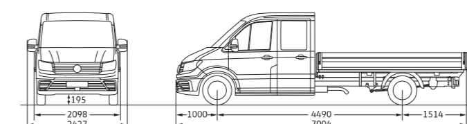
Crafter 50/55 Dual Cab Chassis LWB - with Optional Alloy Tray
