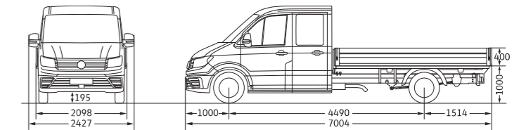
Crafter 35 Dual Cab LWB - with Optional Alloy Tray
