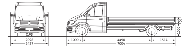
Crafter 35 Single Cab LWB - with Optional Alloy Tray
