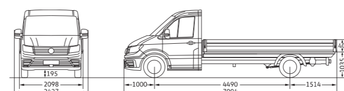
Crafter 50/55 Single Cab Chassis LWB - with Optional Alloy Tray
