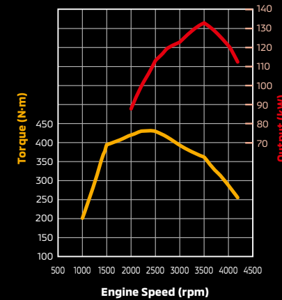
MIVEC Turbo charger High power (133kW//3500rpm)
